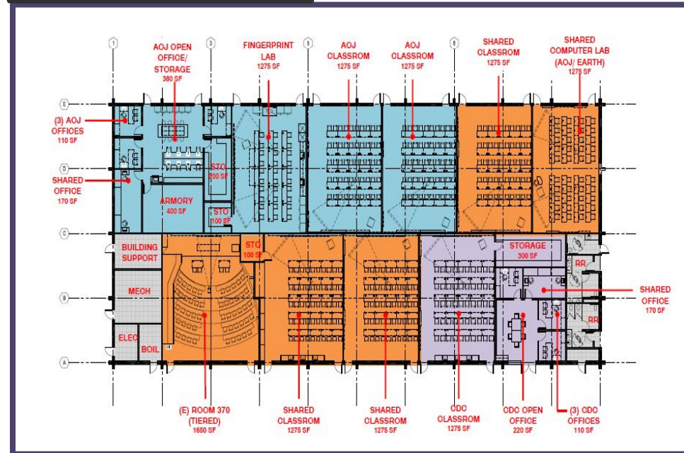
Building 31 Floorplan
